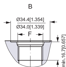
B: UNF main ports F: 7 / 8 - 14 UNF O-ring boss port
