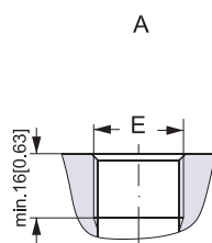
A: G main ports E: ISO 228/1 - G 1 / 2
